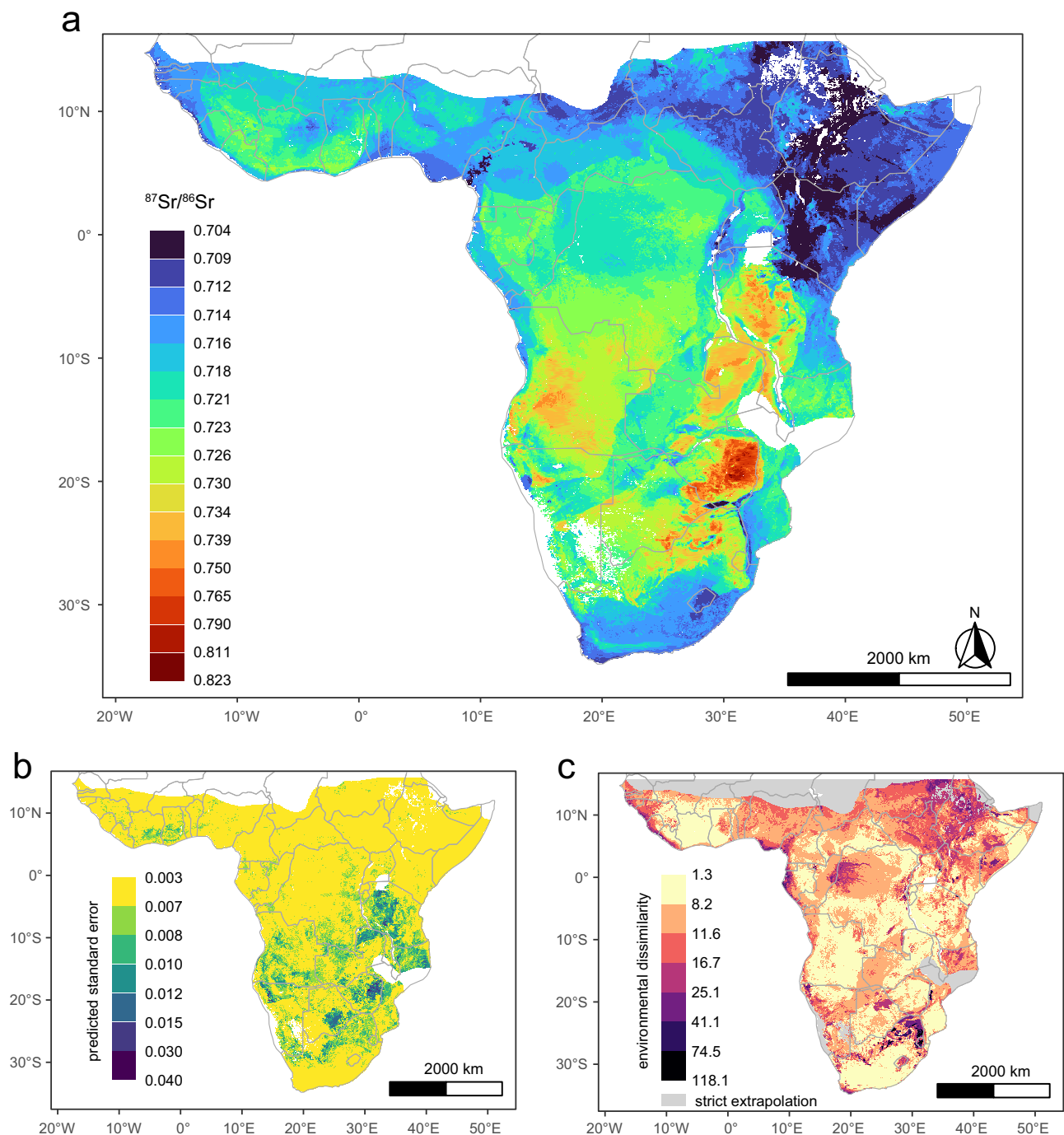
Fig. 2 | Bioavailable strontium isoscape and associated standard error map for sub-Saharan Africa. a Bioavailable strontium isoscape for sub-Saharan Africa. b Standard error map for the strontium isoscape. c Mobility-oriented parity metrics. The multivariate Mahalanobis distance, or environmental similarity metric, relates to the comparison between the calibration dataset and prediction regions 70 . Darker-shaded areas indicate greater dissimilarity from the environmental
